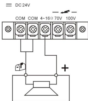
4 Ω speaker connection
