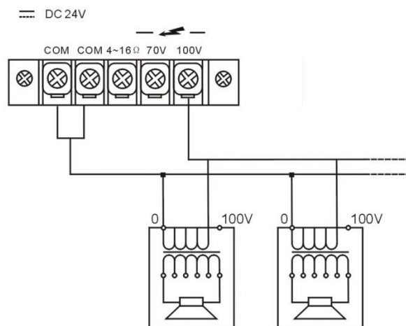
100V connection with a transformer
